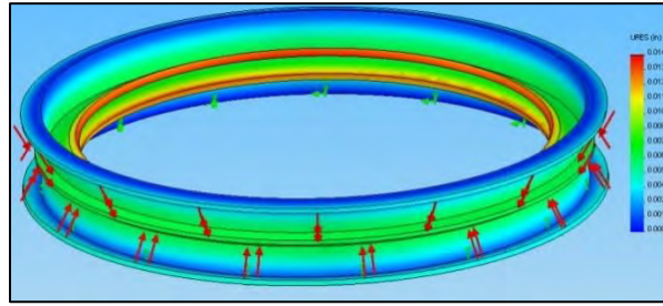
Figure 7-24: FEM simulates a clamp band separation system via radially inward preload from band tension. Warping can result.
